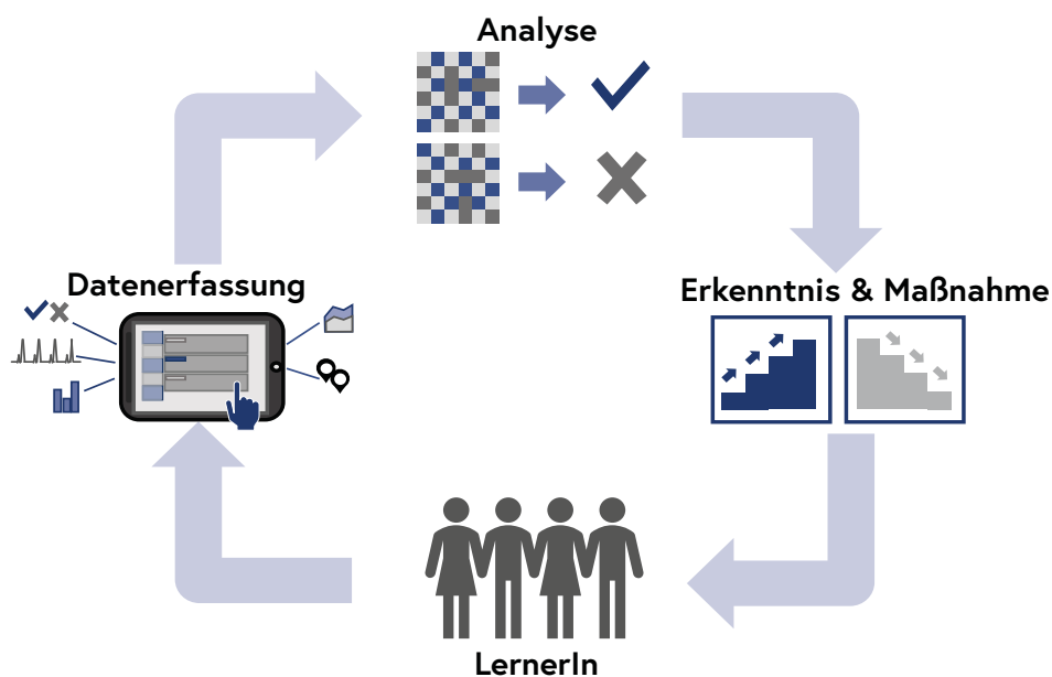
Abb. 5: Hybrides KI-System
