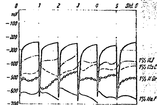
Abb. 3. Ruhepotential des Amalgams in Polyphosphatkalium, in 1% NaF, in 1% KBr, in 1% NaCl und in 1% KI.
