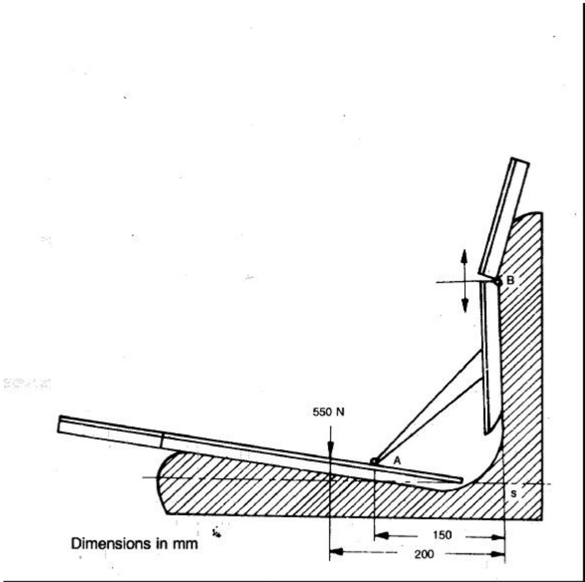
Figure 8 Method of determining seat reference point
