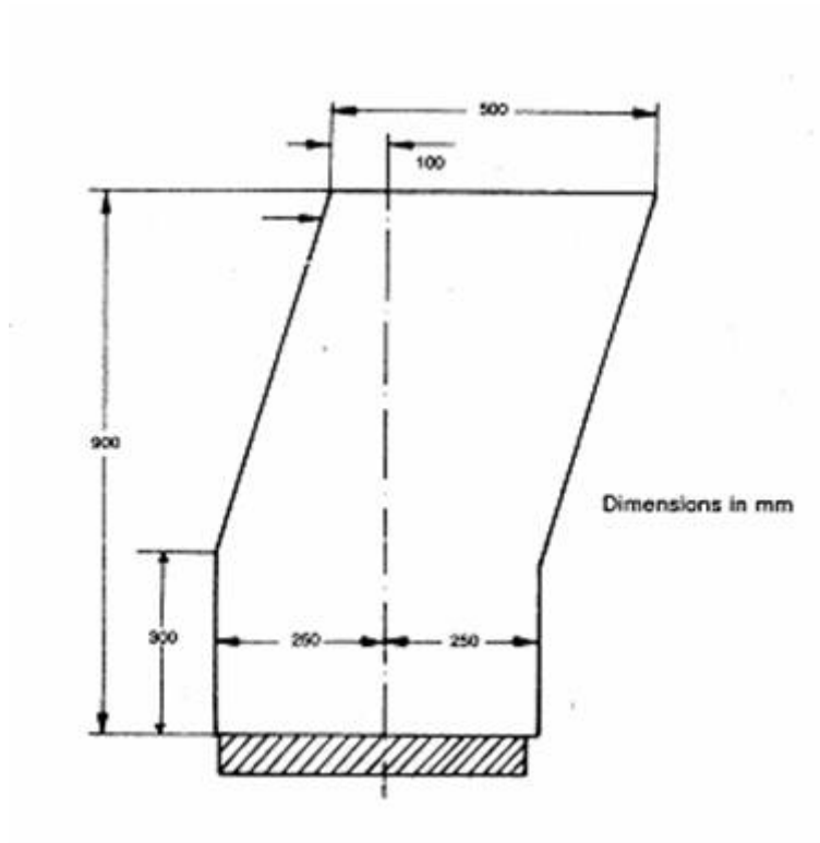
Figure 6b Front/rear view of zone of clearance
