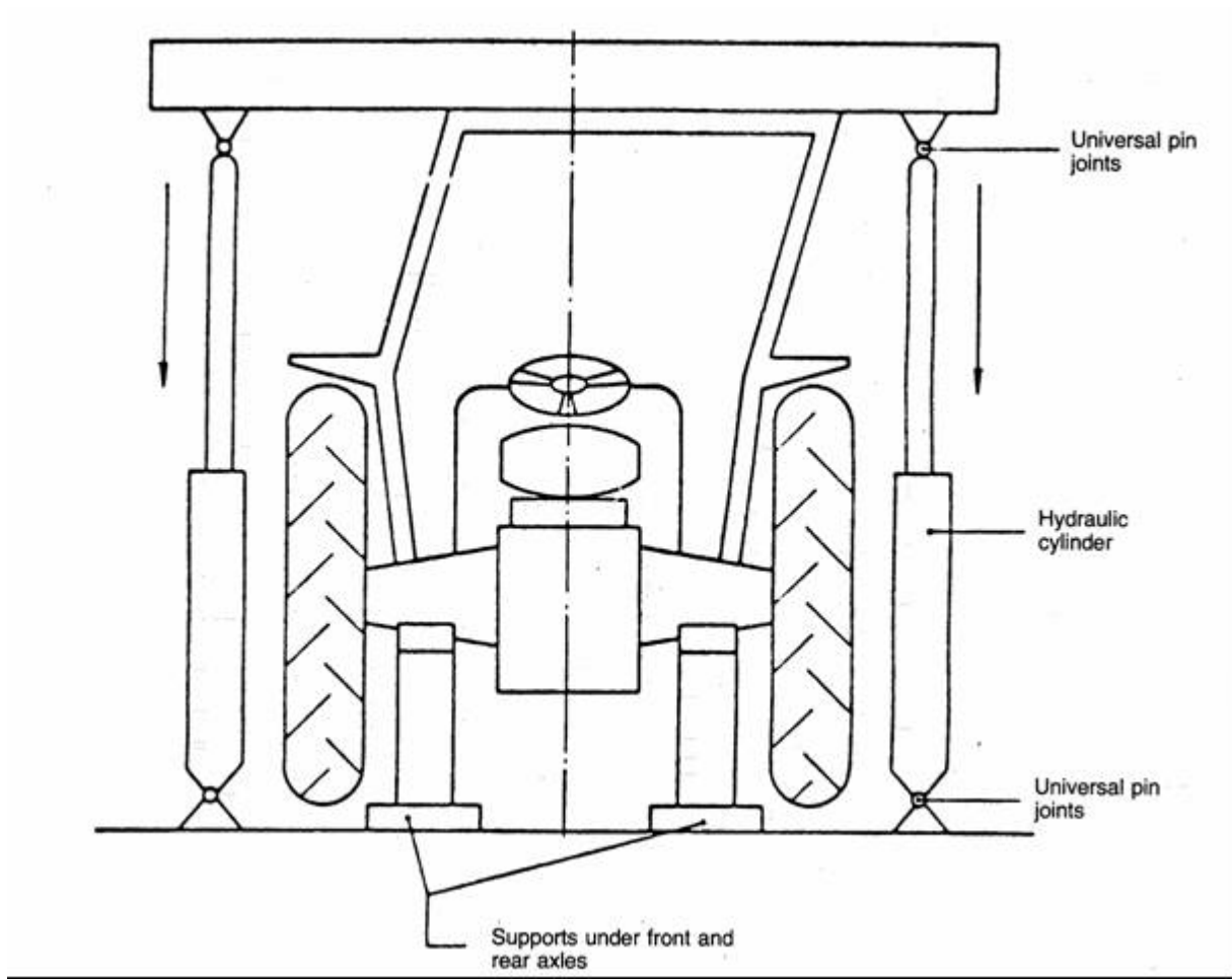
Figure 3 Example of an arrangement for crushing test
