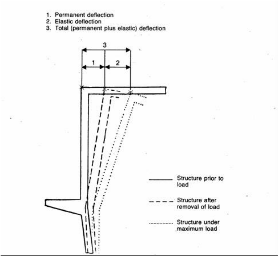
Figure 5 Illustration of the terms permanent, elastic and total deflection
