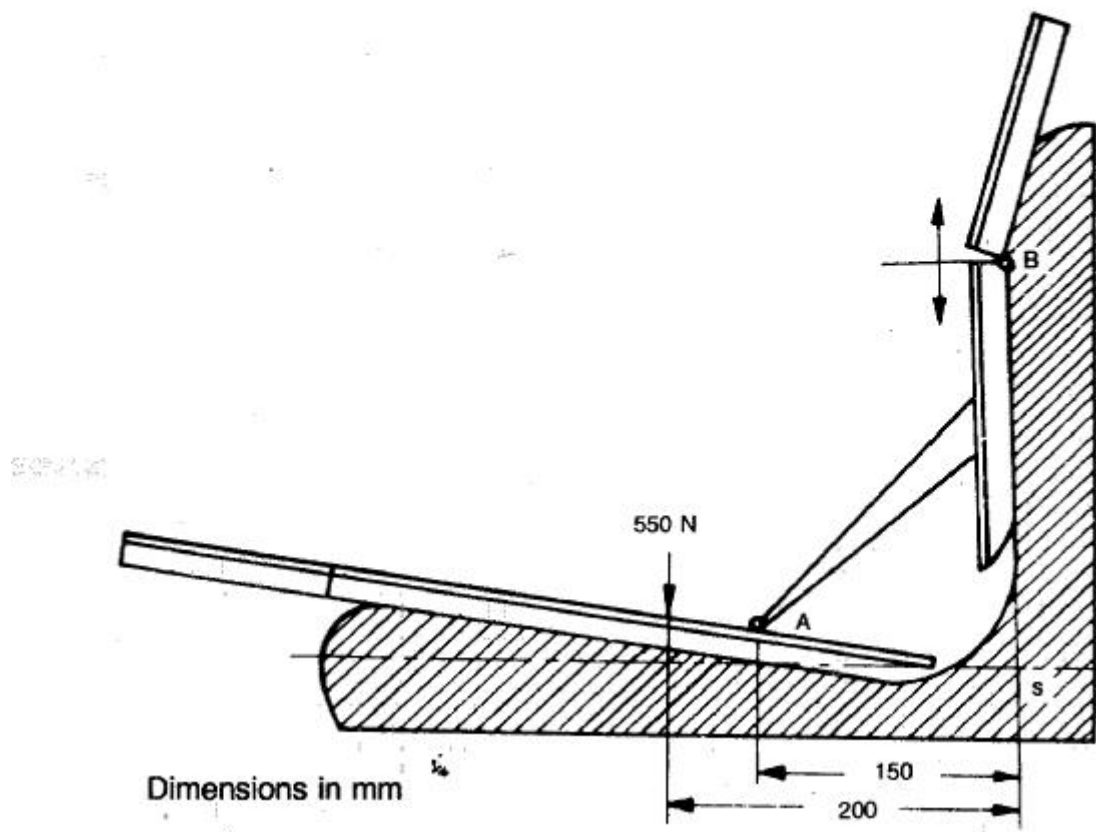
Figure 8 Method of determining seat reference point
