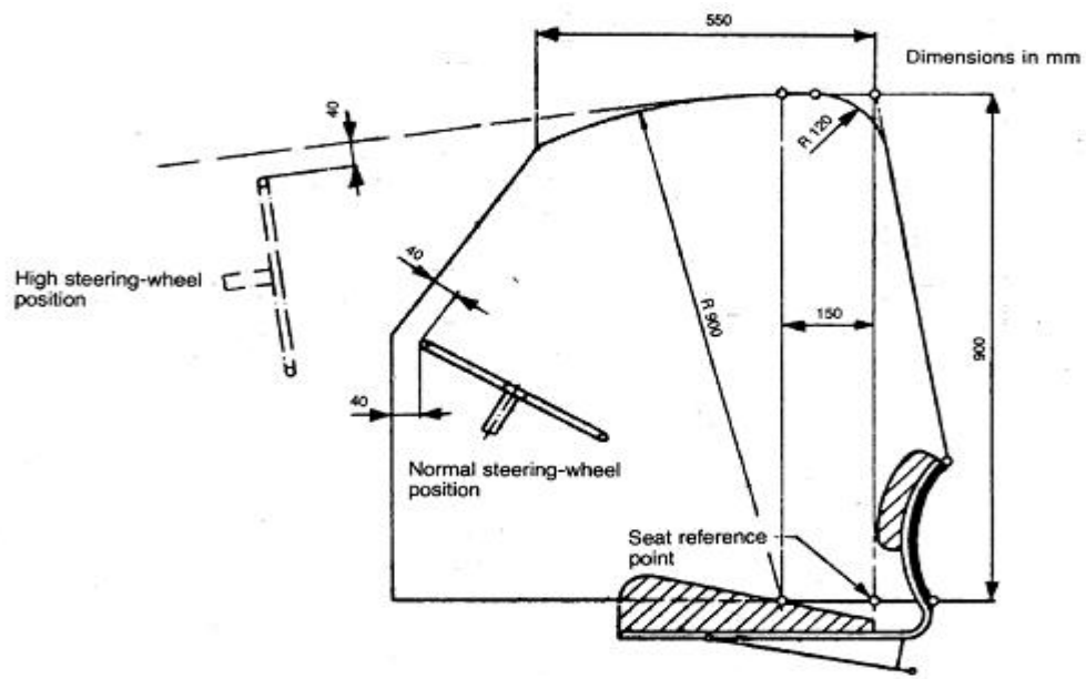
Figure 6a Side view of zone clearance
