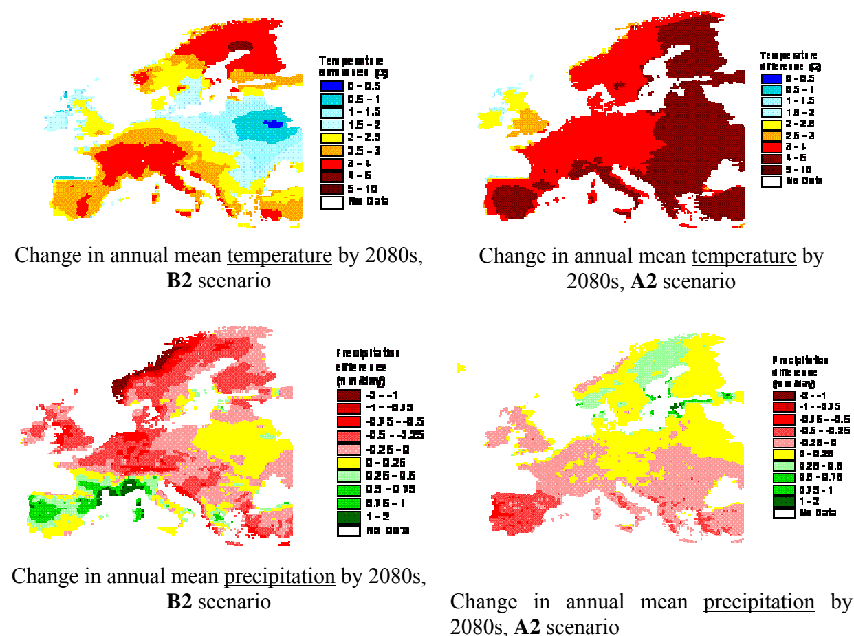
Figure 5: Changes in annual mean temperature and precipitation by 2071-2100 relative to 1961-1990 under the B2 and A2 scenario. Source Prudence, based on HadCM3.
