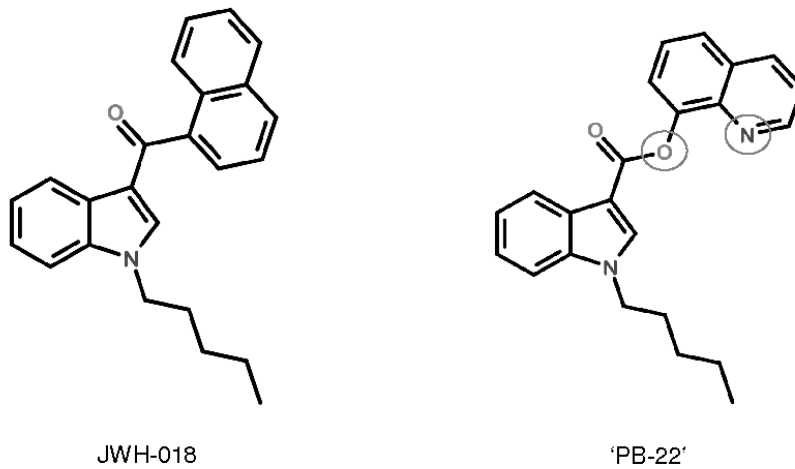
Figure 2. Structure of JWH-018 and 'PB-22'
