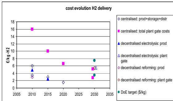
Figure 11.1: Trends in cost reductions for FCH technologies
