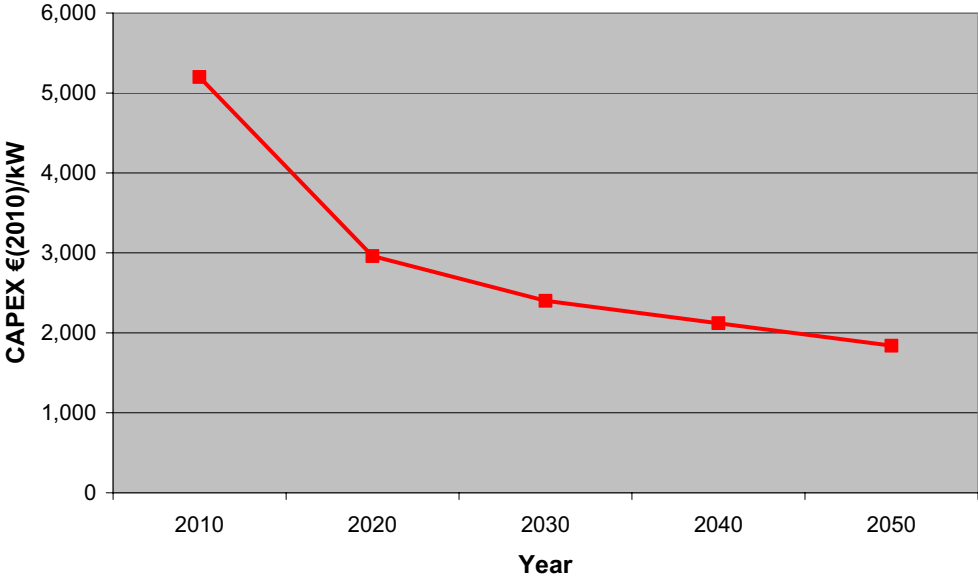
Fig 2: Capital cost estimates to 2050 for concentrated solar power plants.
