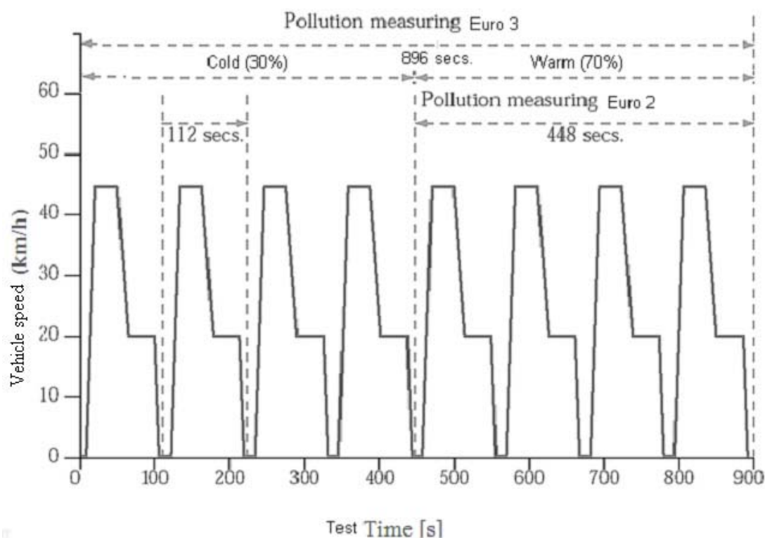
Figure 1: Pollutant emission sampling for Euro 3 as compared with Euro 2 for an L1e, L2e or L6e category vehicle
