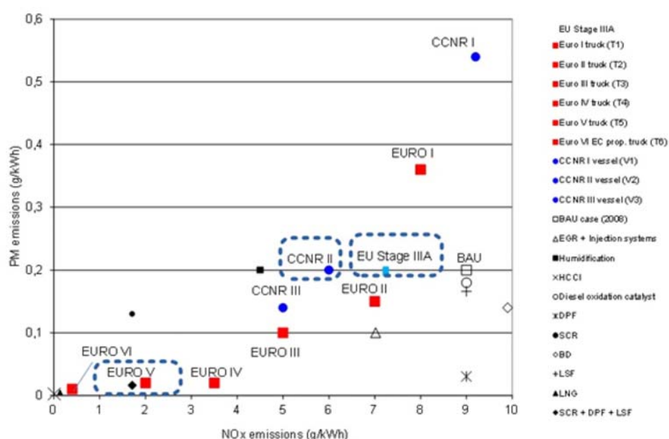
Figure 4: Current emission standards for road transport and IWT: NO x /PM
