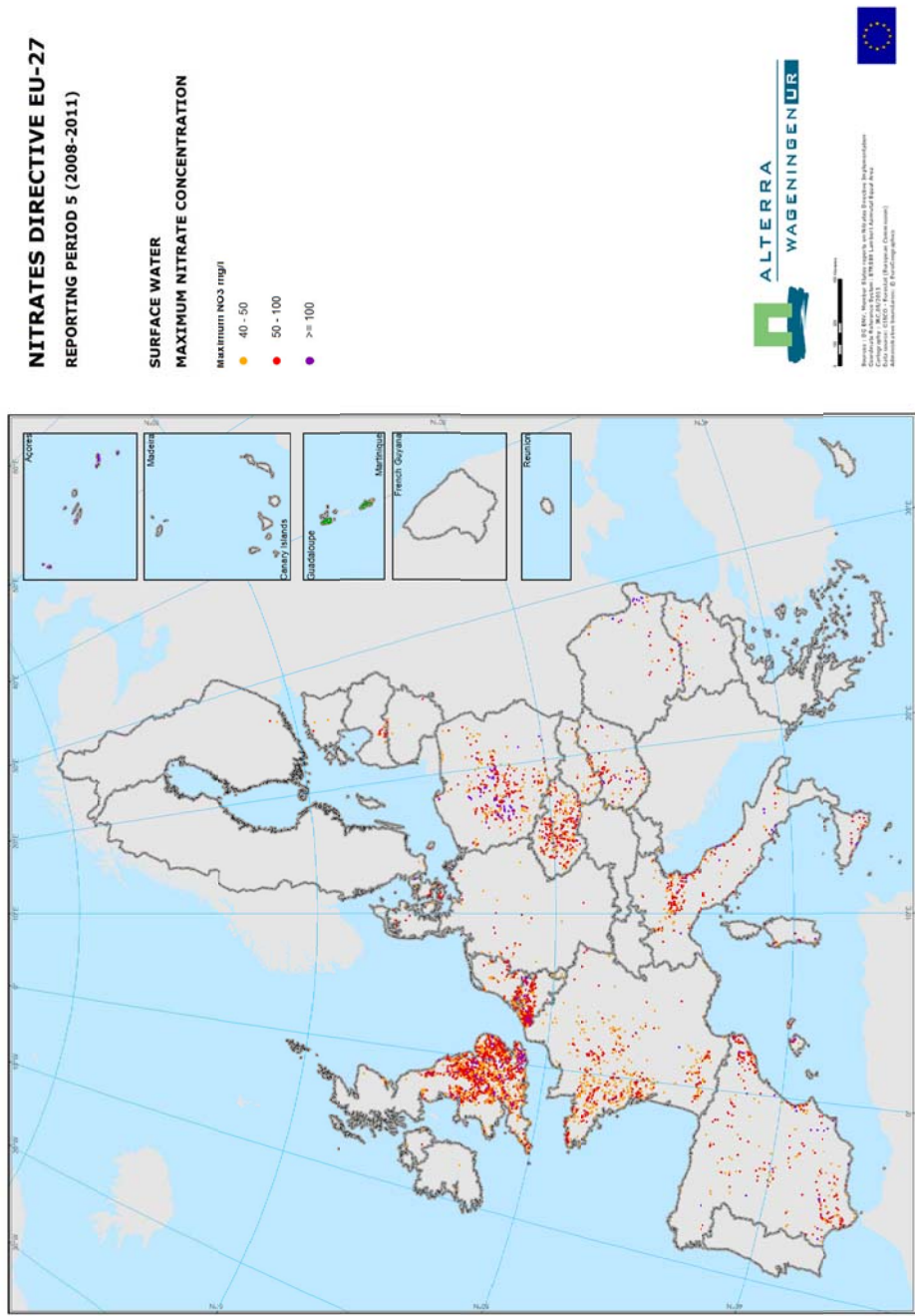
Map 5. Surface fresh water maximum nitrate concentrations for the reporting period 2008-2011.
