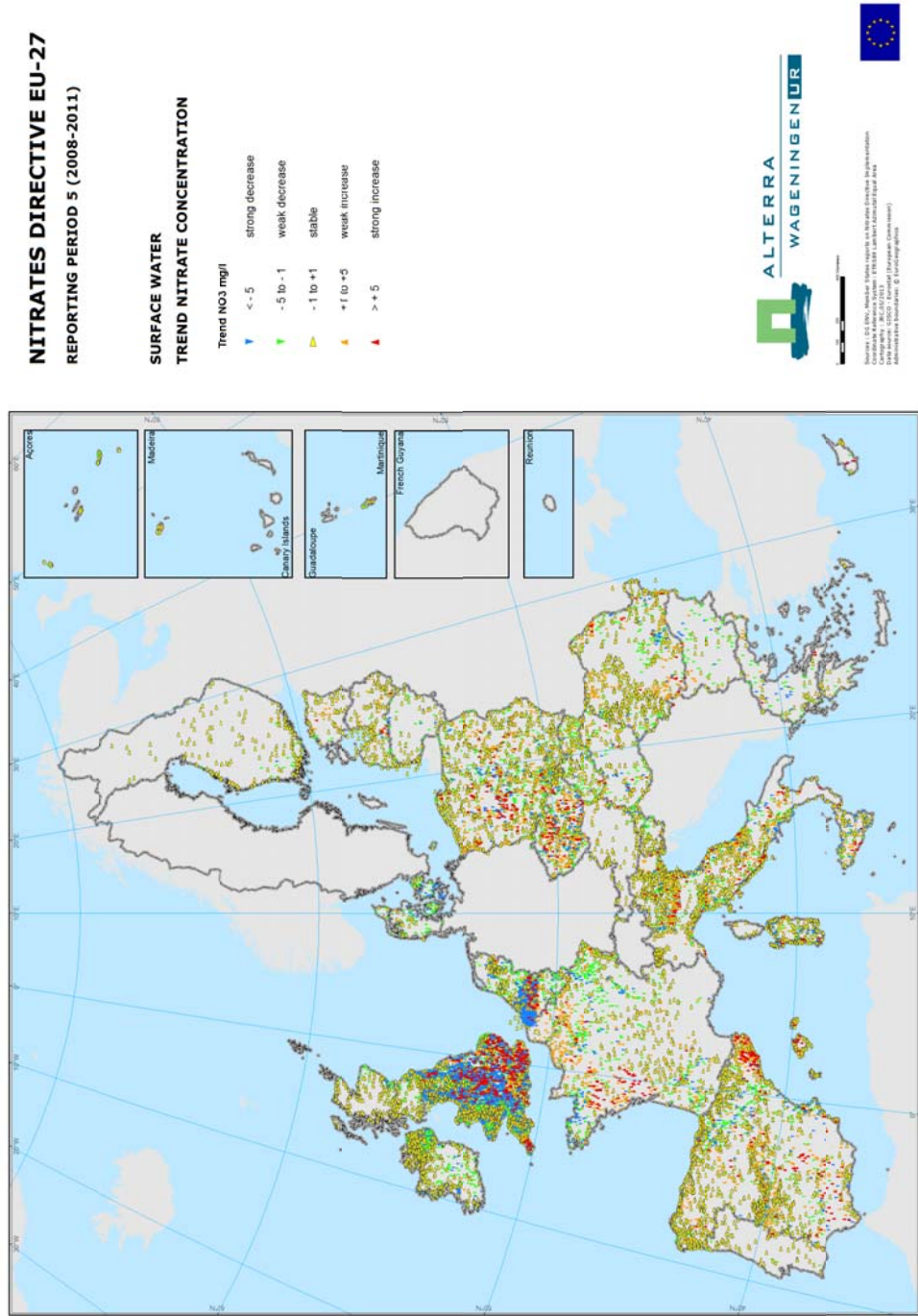
Map 6. Trends in surface fresh water nitrates concentrations between the reporting periods 2004-2007 and 2008-2011.
