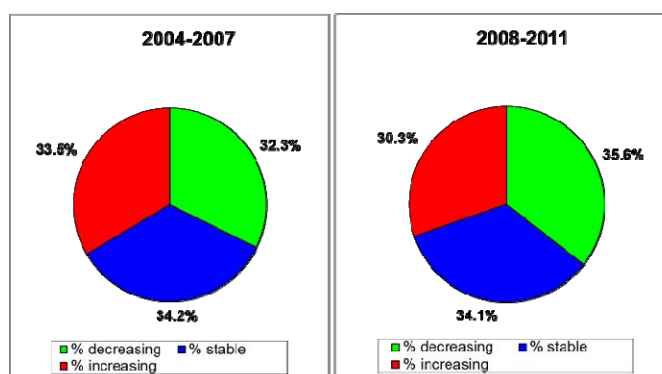
Figure 2. Trends in groundwater nitrate concentrations between the year 2004 and the year 2007 (left) and between the periods 2004-2007 and 2008-2011 (right). A trend between the 2000-2003 and 2004-2007 is not possible, due to a change in the monitoring network in 2004.
