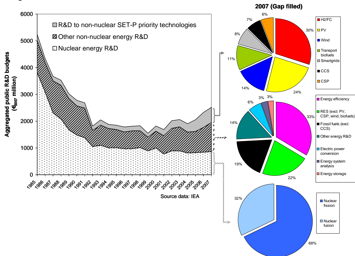
Figure 10: Trends in the aggregated public energy R&D funding of EU Member States (1985-2007; excluding EU funds) and detailed breakdown for the year 2007
