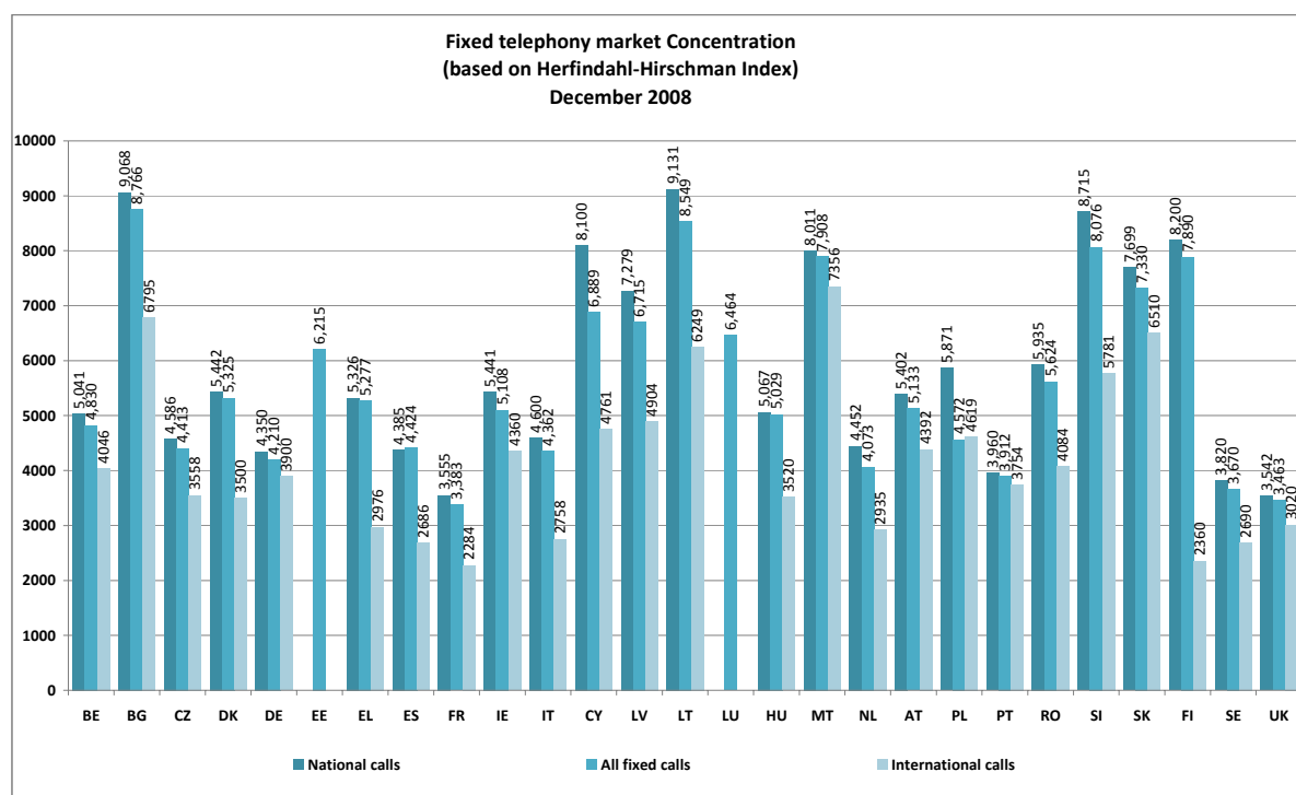
Figure 31: Herfindhal-Hirschman Index
