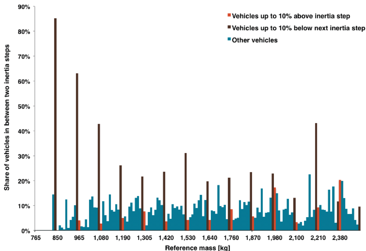
Figure 3 Distribution of vehicles in between inertia steps
