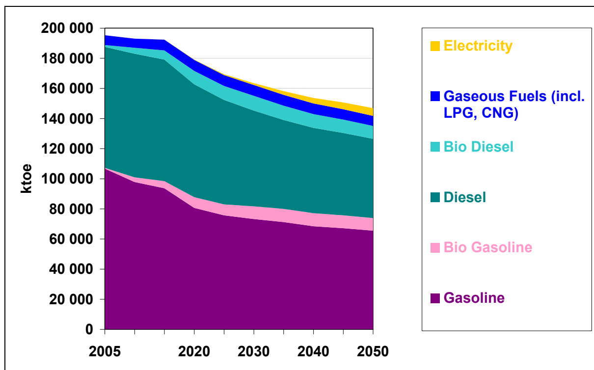
Figure 9: Energy use of light duty vehicles (cars & vans) by fuel
