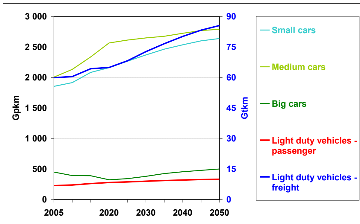
Figure 7: Transport activity of light duty vehicles (cars & vans)
