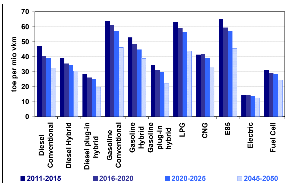
Figure 6: Real world efficiency of new medium sized passenger cars in Scenario 0
