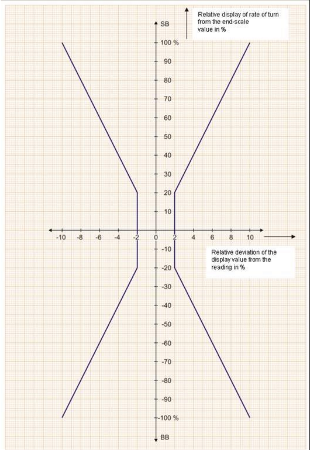
Figure 1: Maximum tolerances for indication errors of rate-of-turn indicators
