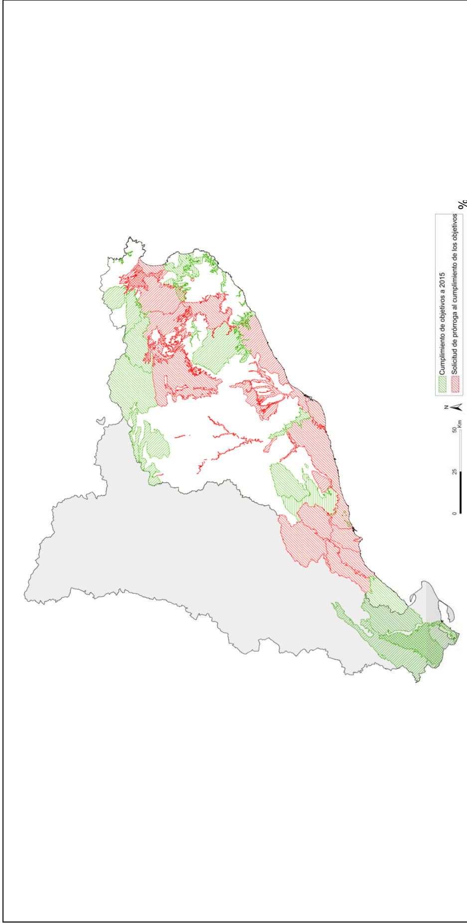
Figure 6.3: Expected fulfilment of objectives in 2015 (groundwater) Source:RBMP
