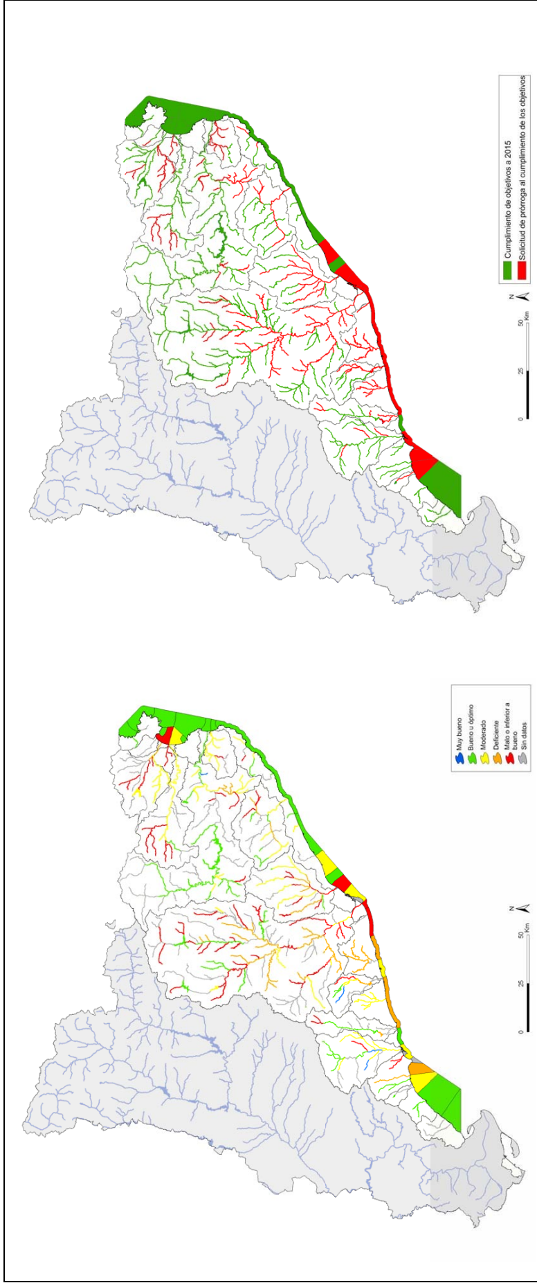
Figure 6.1: (left) Status in 2008; (right) Expected fulfillment of objectives in 2015 (surface water) Source: RBMP
