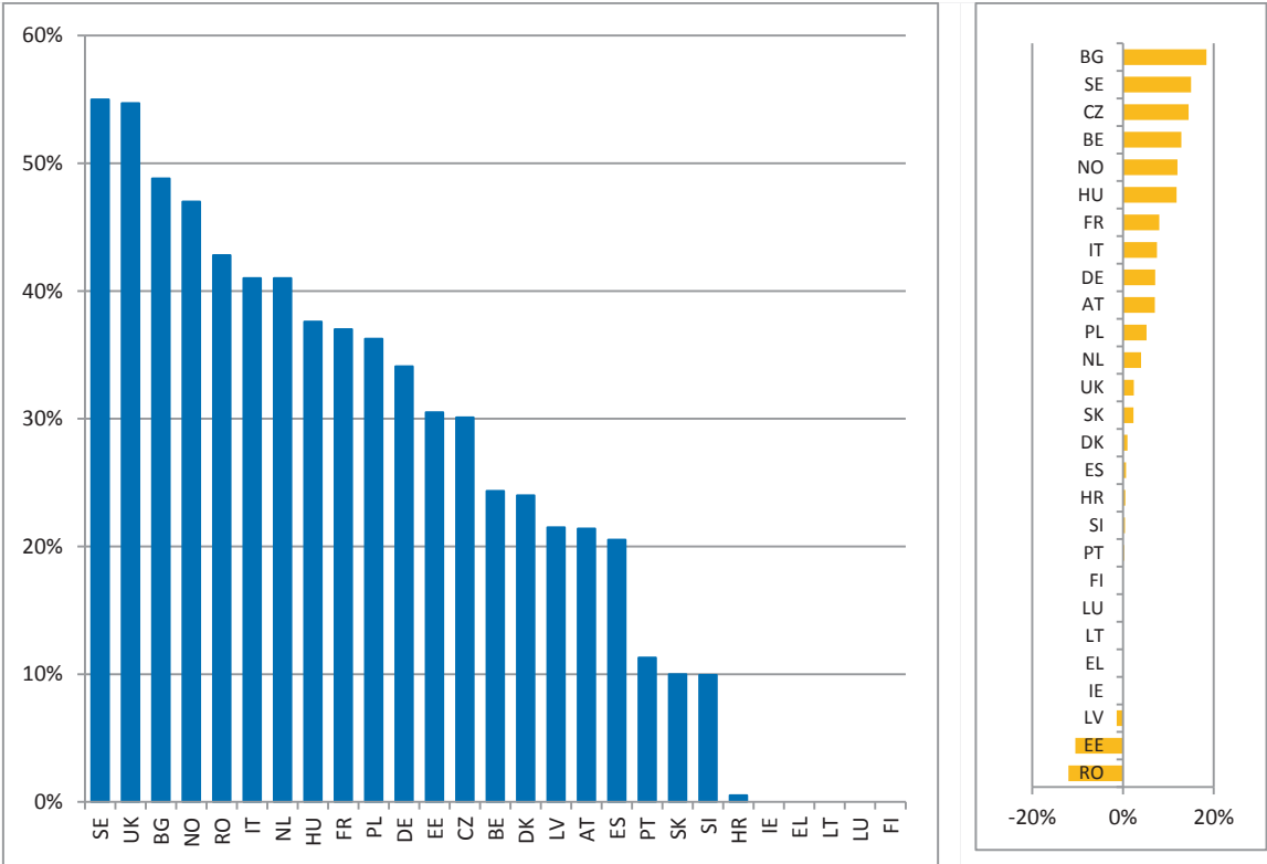
Figure 66 – Market share of competitors in the freight market (2014, % of t-km) and evolution 2011-2014 (in percentage points)
