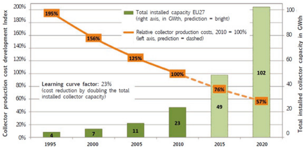
Figure 8: Costs for high-efficient flat plate solar collector panel (of about 2.2 to 2.5 m 2 gross collector area) manufactured in Europe 217
