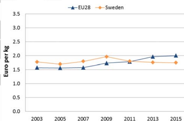
Figure 1: Resource productivity 2003-15 9
