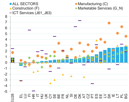
Graph 4.4.4: Labour productivity, 2006-2015
