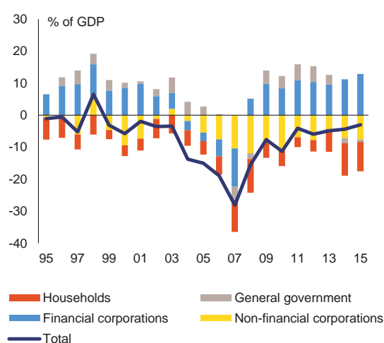
Graph 4.4.1: Savings-investment balance
