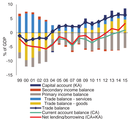
Graph 1.9: Current and capital accounts
