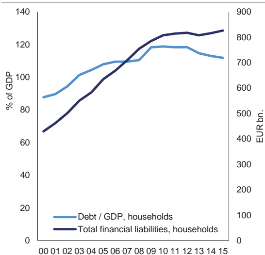
Graph 4.2.4: Household debt
