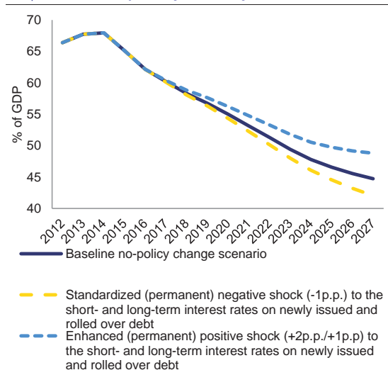
Graph 4.1.3: Debt profile (2012-2027)
