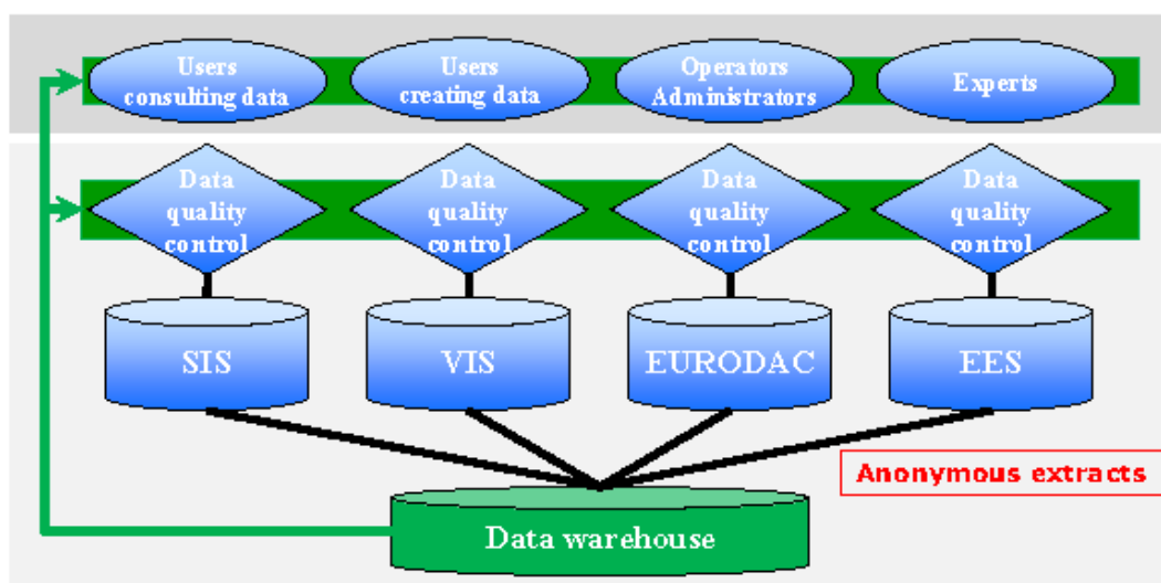
Figure 2 Data warehouse
