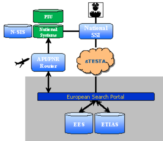
Figure 13 A centralized router for API data
