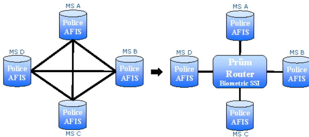
Figure 6 Migration towards a 'hub-and-spoke' centralised Prüm router
