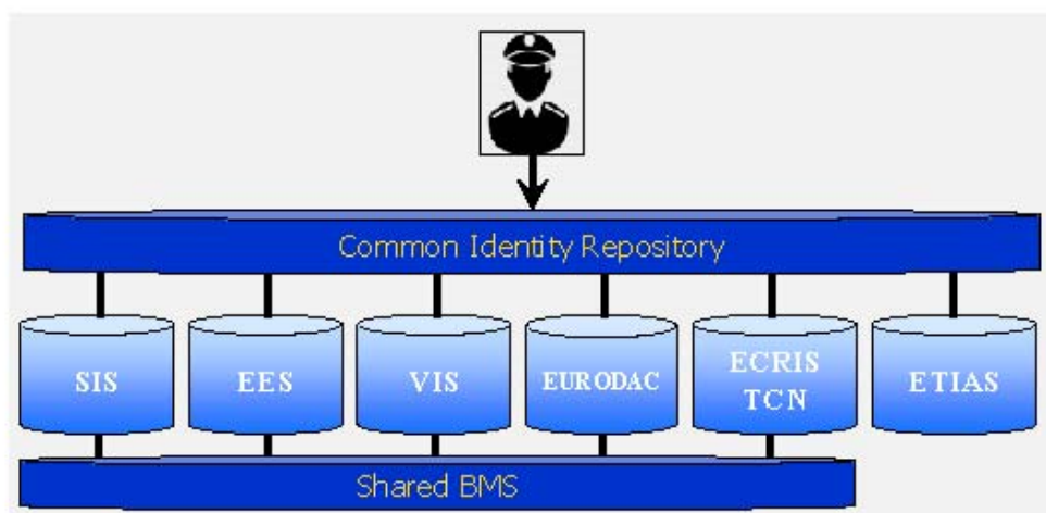
Figure 11 Conceptual view of a common identity repository
