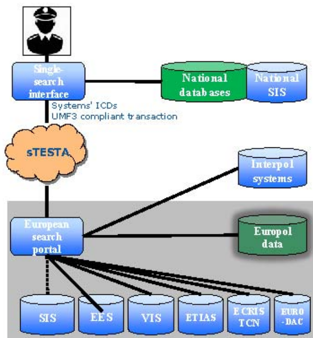
Figure 9 Conceptual view of a European search portal
