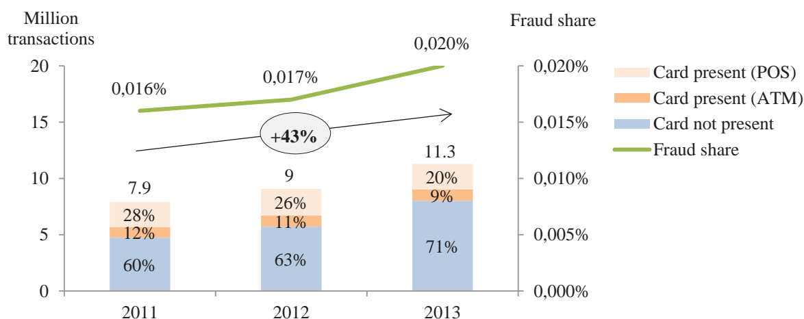
Figure 6: evolution of the total volume of card fraud using cards issued within SEPA 45
