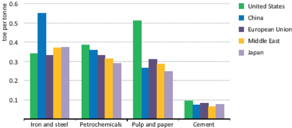
Figure 130. Energy intensity by sub-sector and region, 2011
