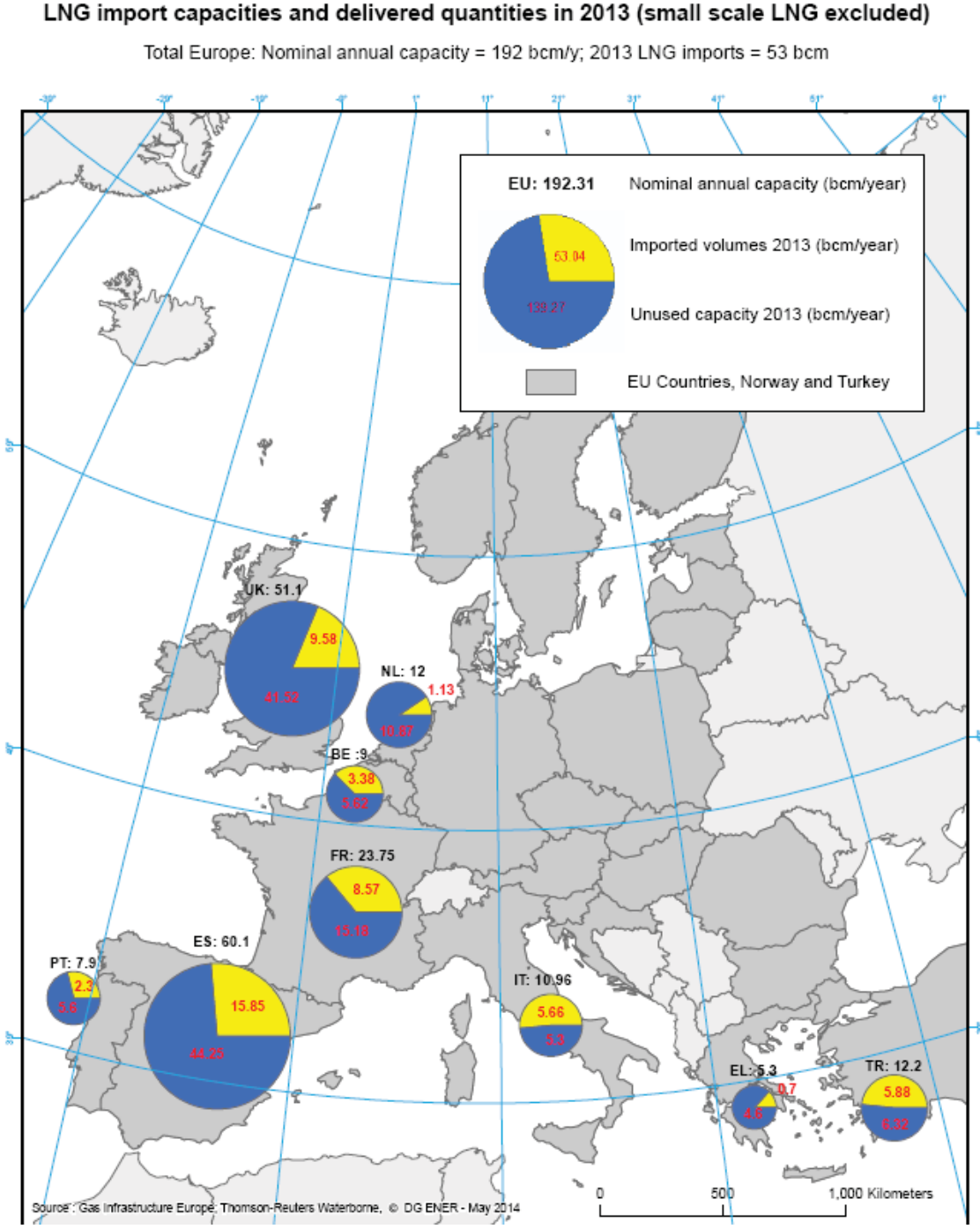
Figure 39. LNG import capacities and delivered quantities in the EU, 2013
