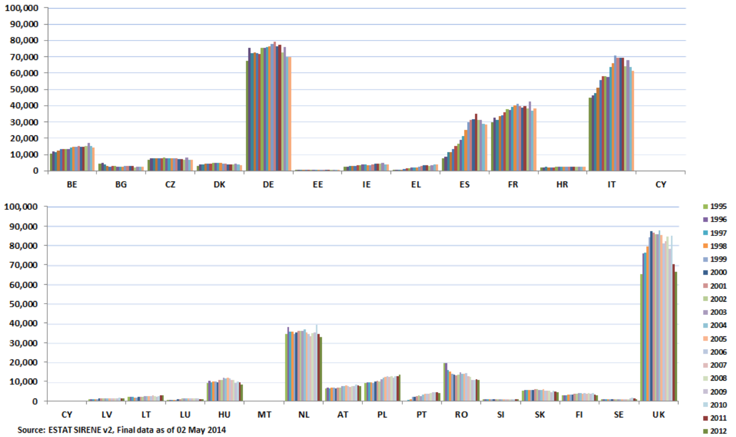
Figure 31. Total production of natural gas in the EU, 1995-2012, ktoe
