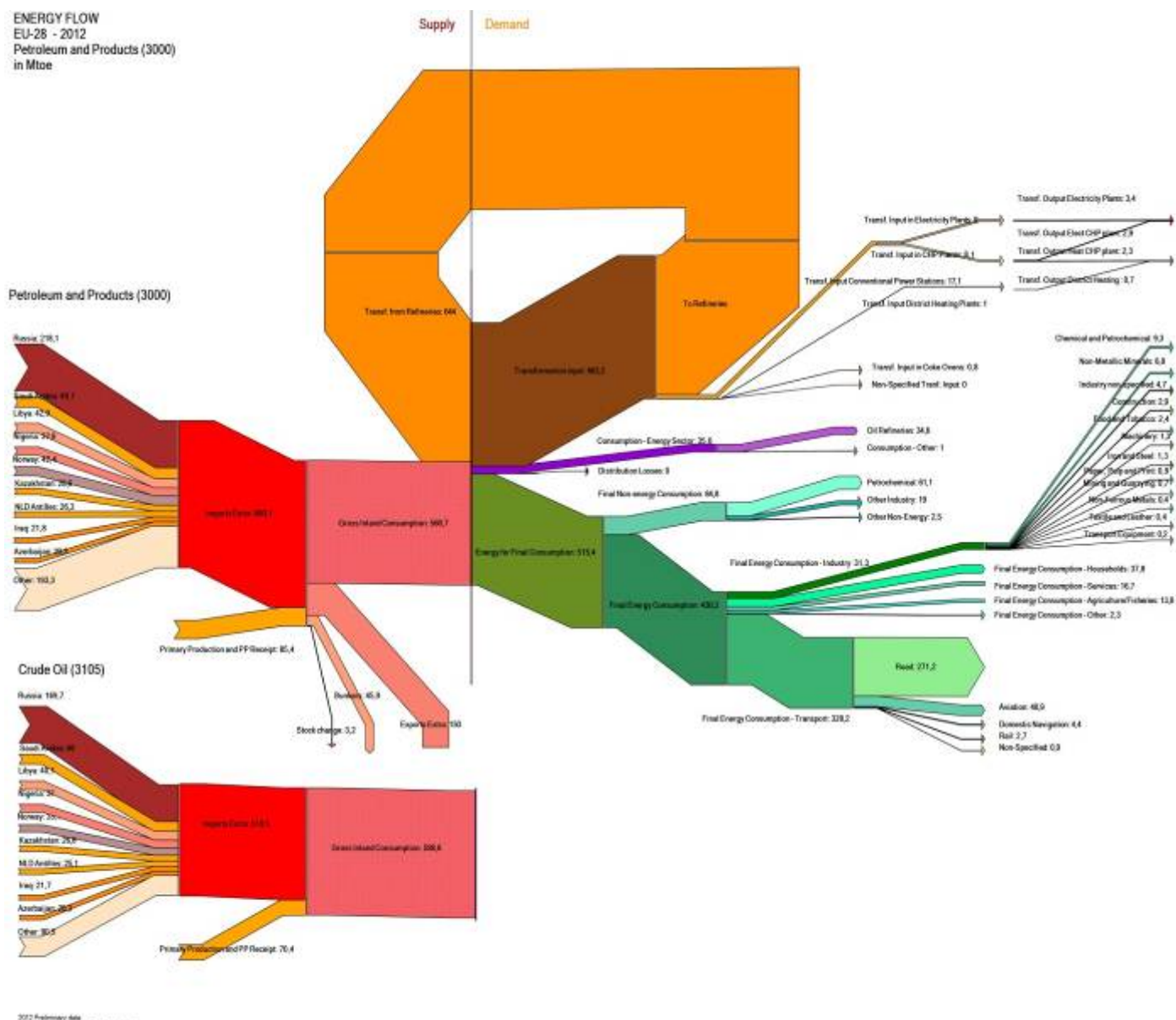
Figure 15. Energy flow of petroleum and products in the EU, 2012
