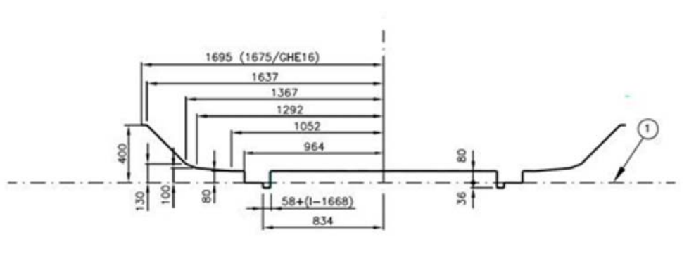
Figure 13: Reference profile of lower parts of kinematic gauge GEI2 for vehicles which may pass over rail brakes in a non-active position ( l =track gauge).
