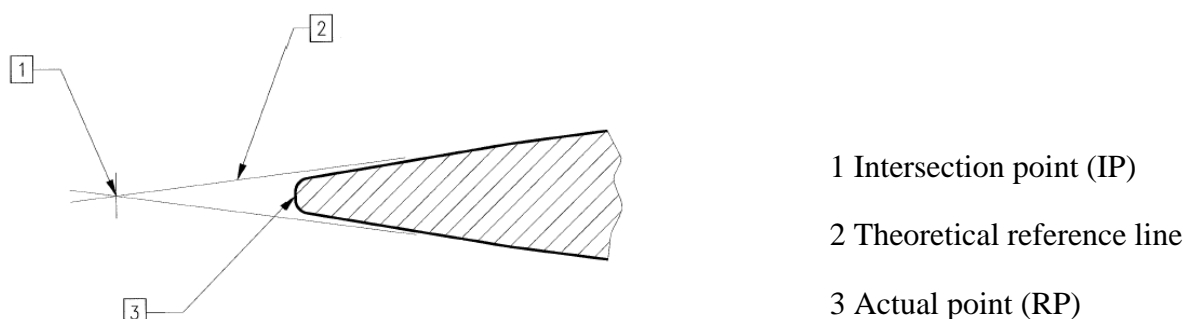
Figure 2: Point retraction in fixed common crossings
