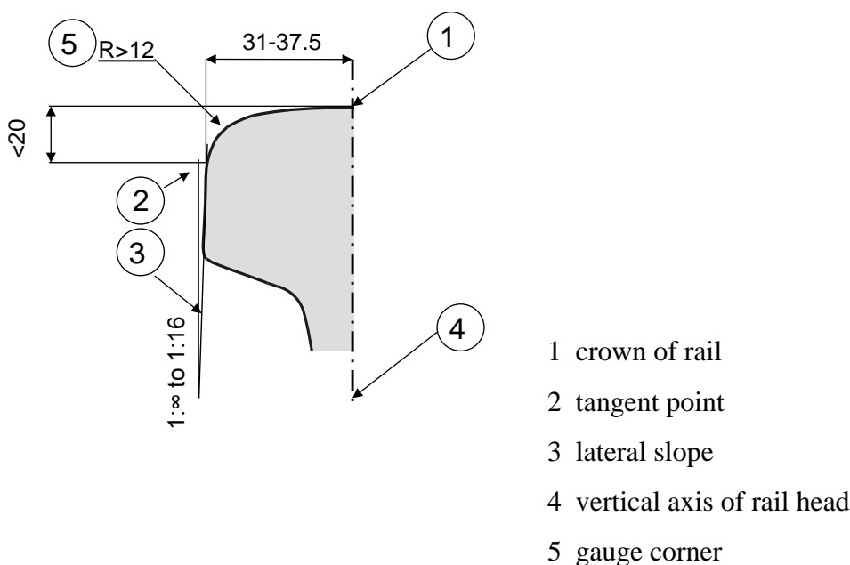
Figure 1: Railhead profile
