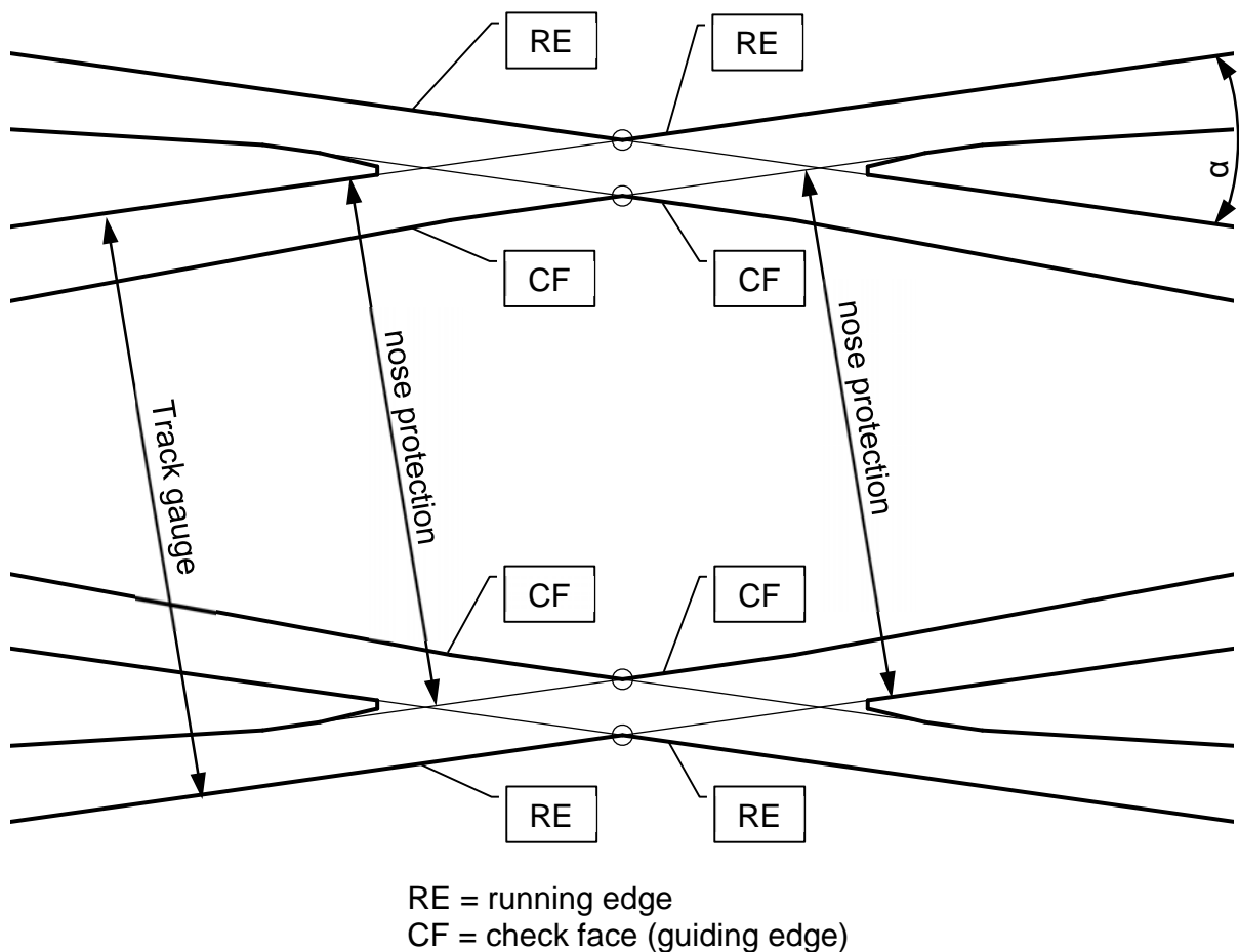
Figure 6: Obtuse crossing
