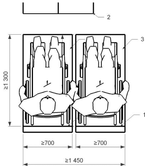
Figure I3 - Two facing wheelchair spaces
