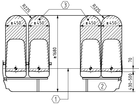
Figure H1 - Priority seat headroom
