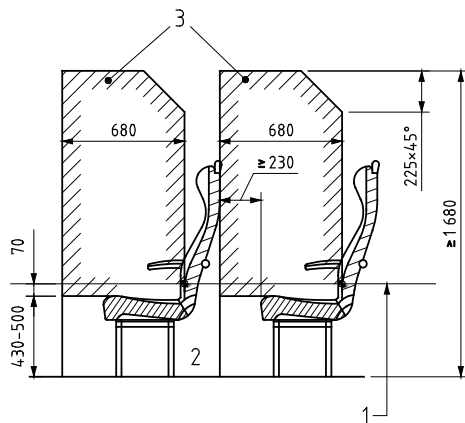
Figure H2 - Unidirectional priority seats
