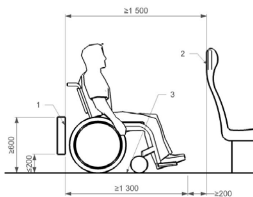
Figure I1 - Wheelchair space in facing seating arrangement
