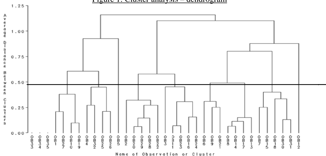
Figure 1: Cluster analysis – dendrogram
