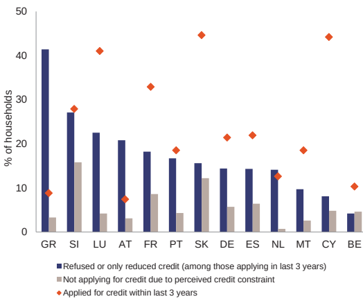
Graph 2.4.12: Credit constraints (2010)
