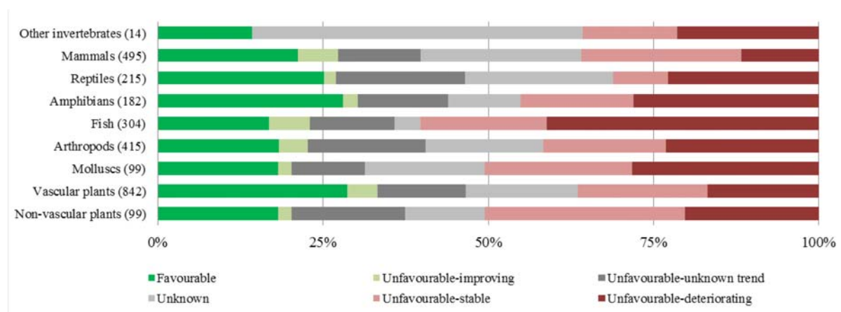
Figure 5 — Conservation status of and trends for species per taxonomic group
