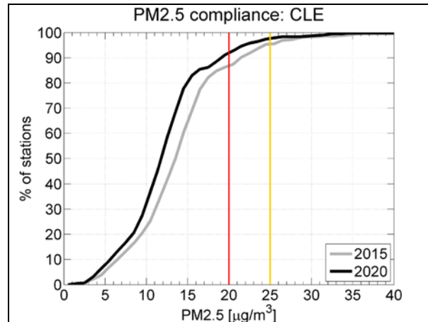
Figure 1: Projected compliance with PM 2.5 limit values (2015 and 2020) assuming no change to current policies
