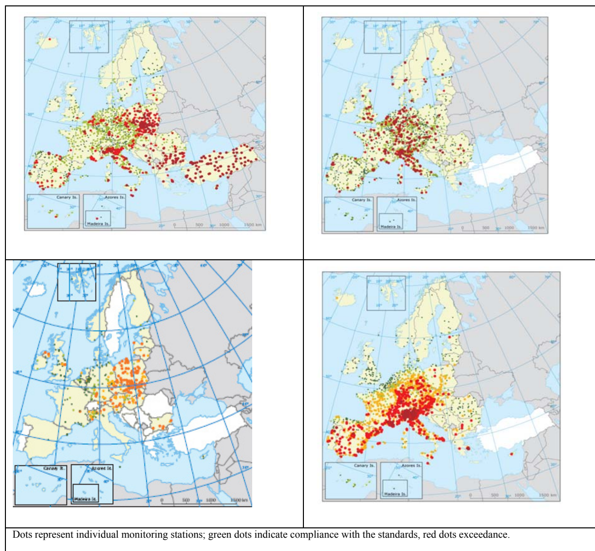
Figure 6: Exceedance of EU air quality standards in 2010 for PM 10 , NO 2 , Ozone, and BaP (clockwise from upper right) in 2010 (EEA)
