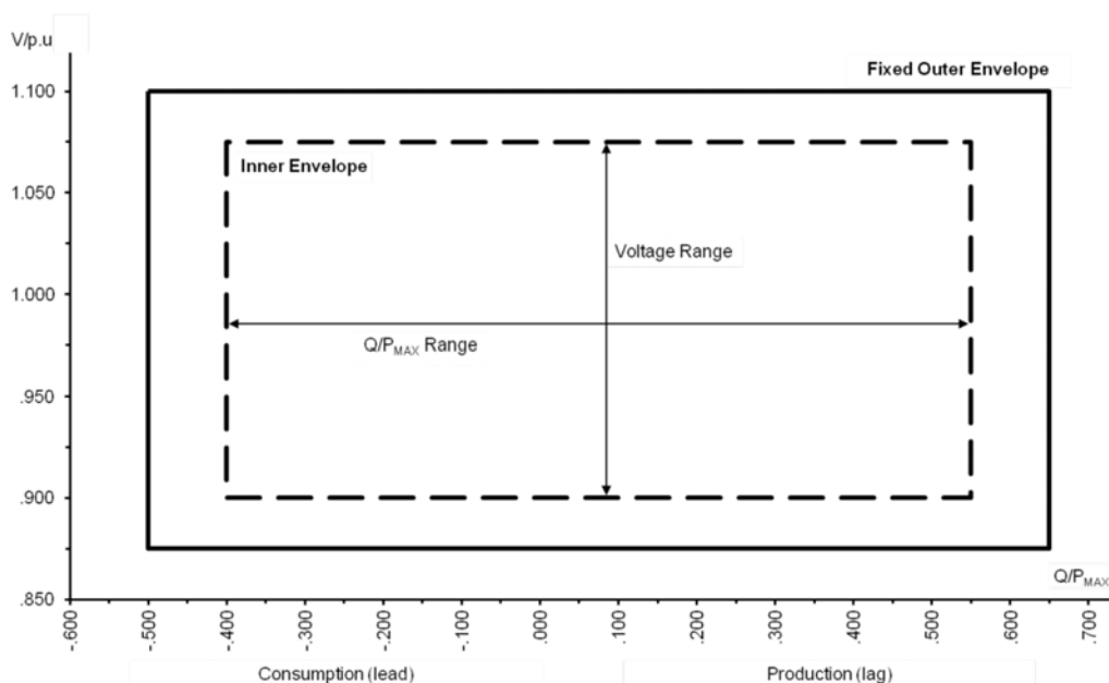
Figure 7: U - Q/P_{\max} -profile of a synchronous power generating module. The diagram represents boundaries of a U - Q/P_{\max} -profile by the voltage at the connection point, expressed by the ratio of its actual value and the reference 1 pu value, against the
