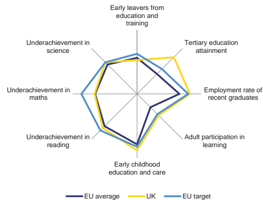
Graph 3.2.5: Education indicators
