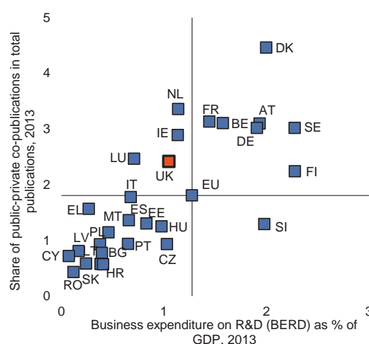
Graph 3.3.4: Public-private co-publication
