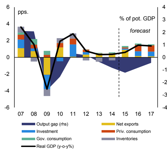
Graph 1.4: Real GDP growth and contributions, output gap
