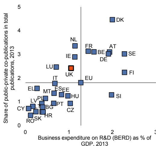
Graph 3.3.4: Public-private co-publication
