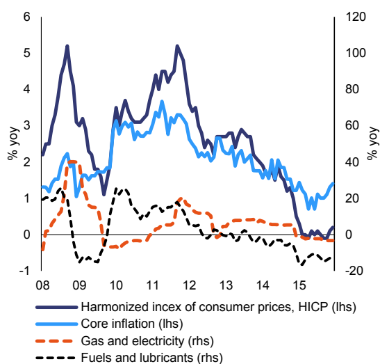
Graph 1.6: Price indicators
