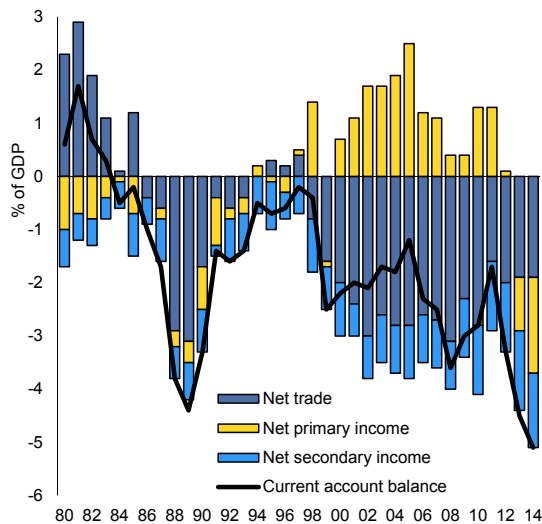
Graph 1.12: Current account
