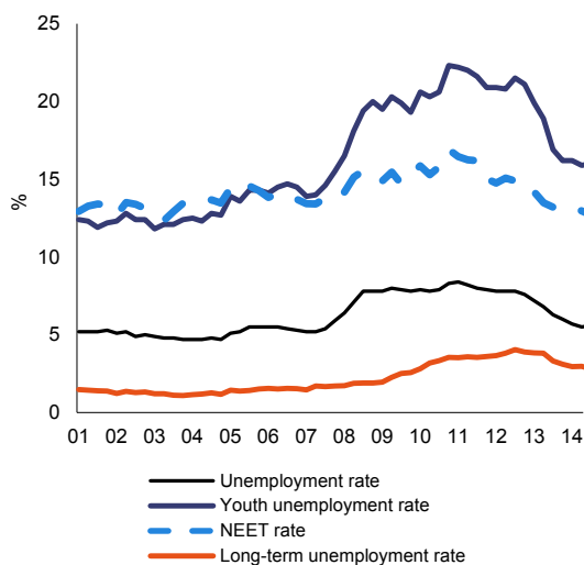
Graph 3.2.1: Employment trends
