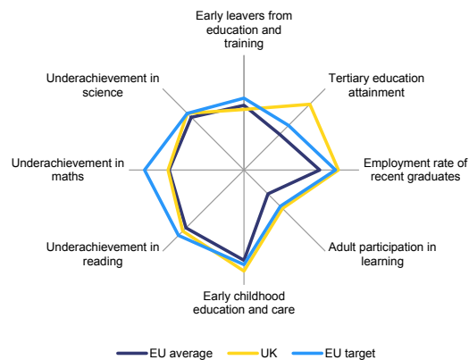
Graph 3.2.5: Education indicators
