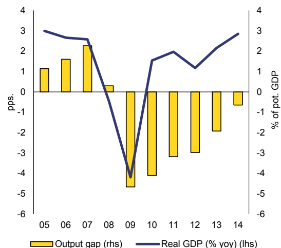
Graph 1.9: Output gap
