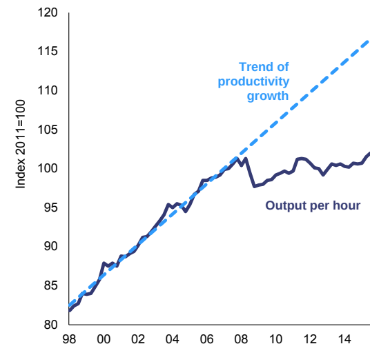
Graph 3.3.1: Productivity
