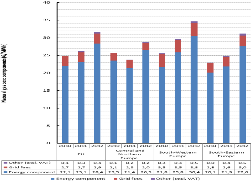
Figure 23 Components of the natural gas bills paid by the 12 sampled wall and floor tiles producers in Europe (€/MWh)
