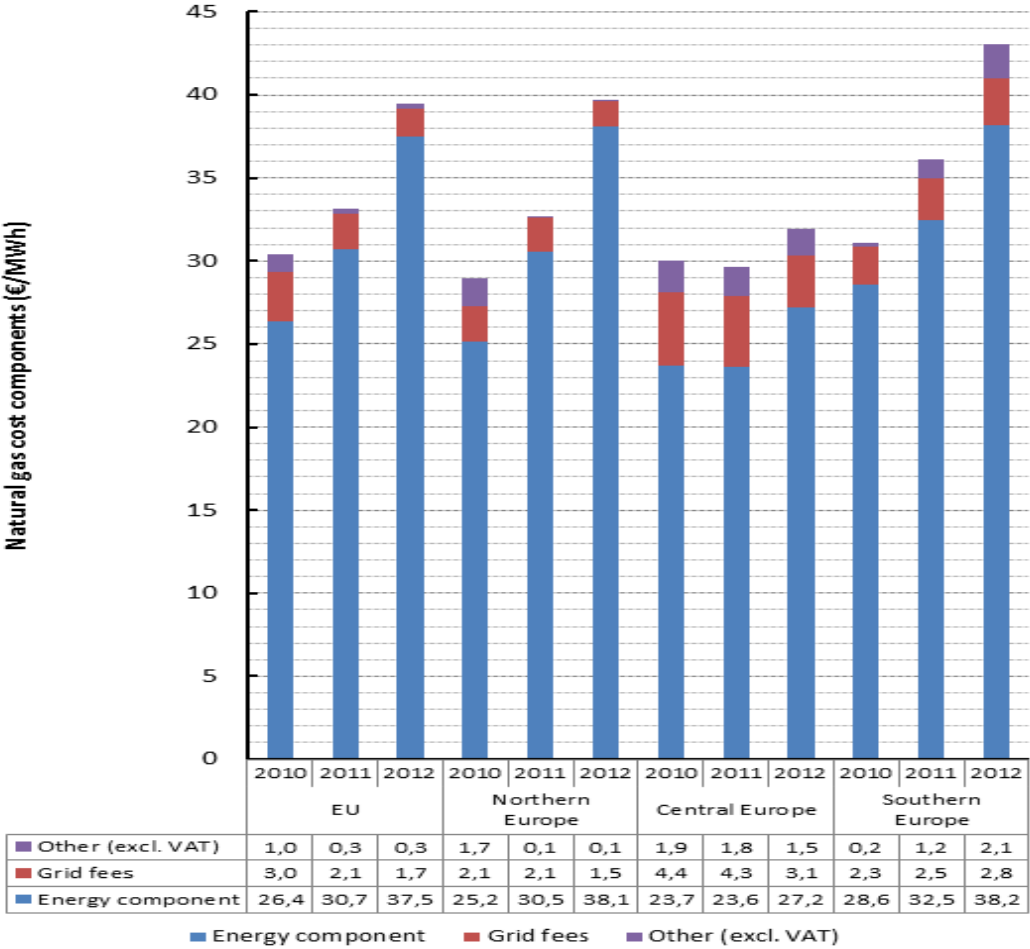
Figure 20 Components of the natural gas bills paid by the 13 sampled bricks and roof tiles producers in Europe (€/MWh)
