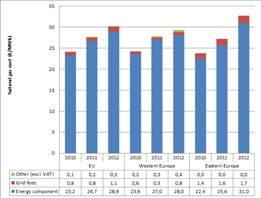
Figure 26 Components of the natural gas bills paid by the 10 sampled float glass producers in Europe (€/MWh)
