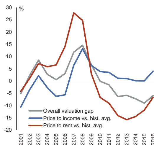
Graph 3.2.1: Overvaluation gap
