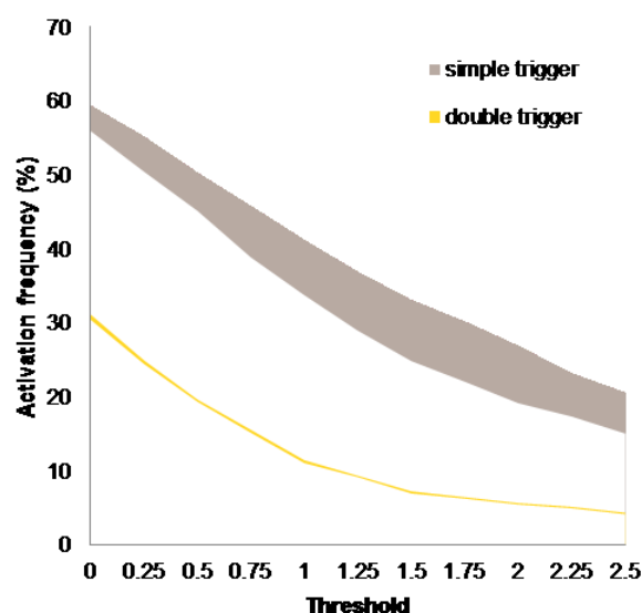
Figure 19: Frequency of activation depending on the threshold
