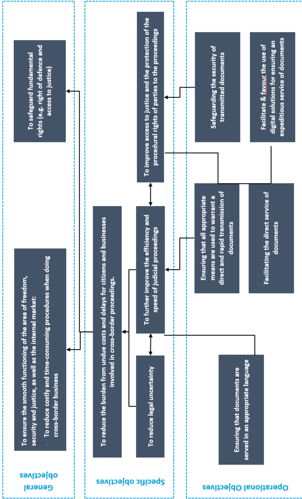
Figure 2: Objectives Tree
