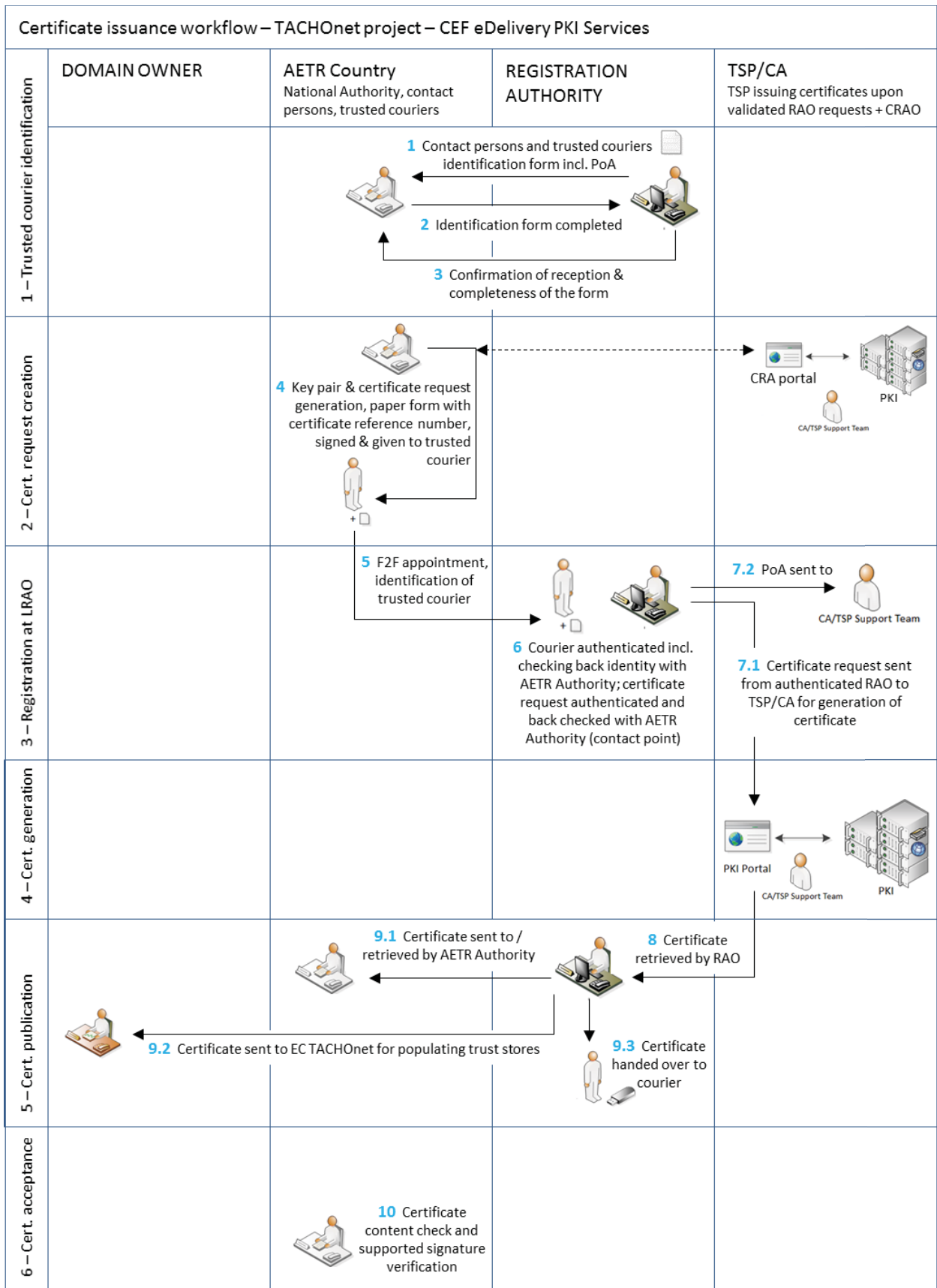
Figure 1 - Certificate issuance workflow
