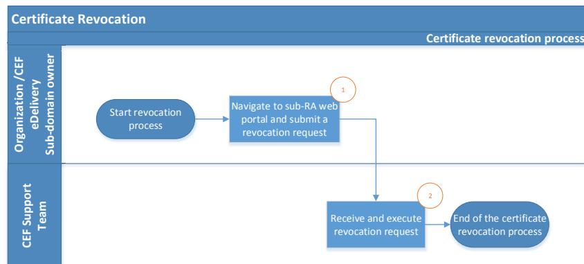
Figure 13 - Certificate revocation
