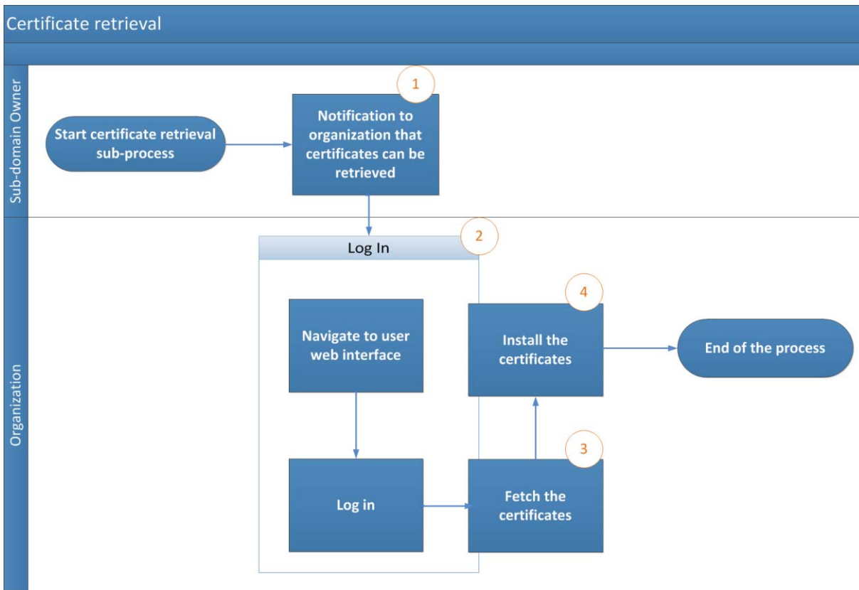
Figure 12 - Certificate retrieval
