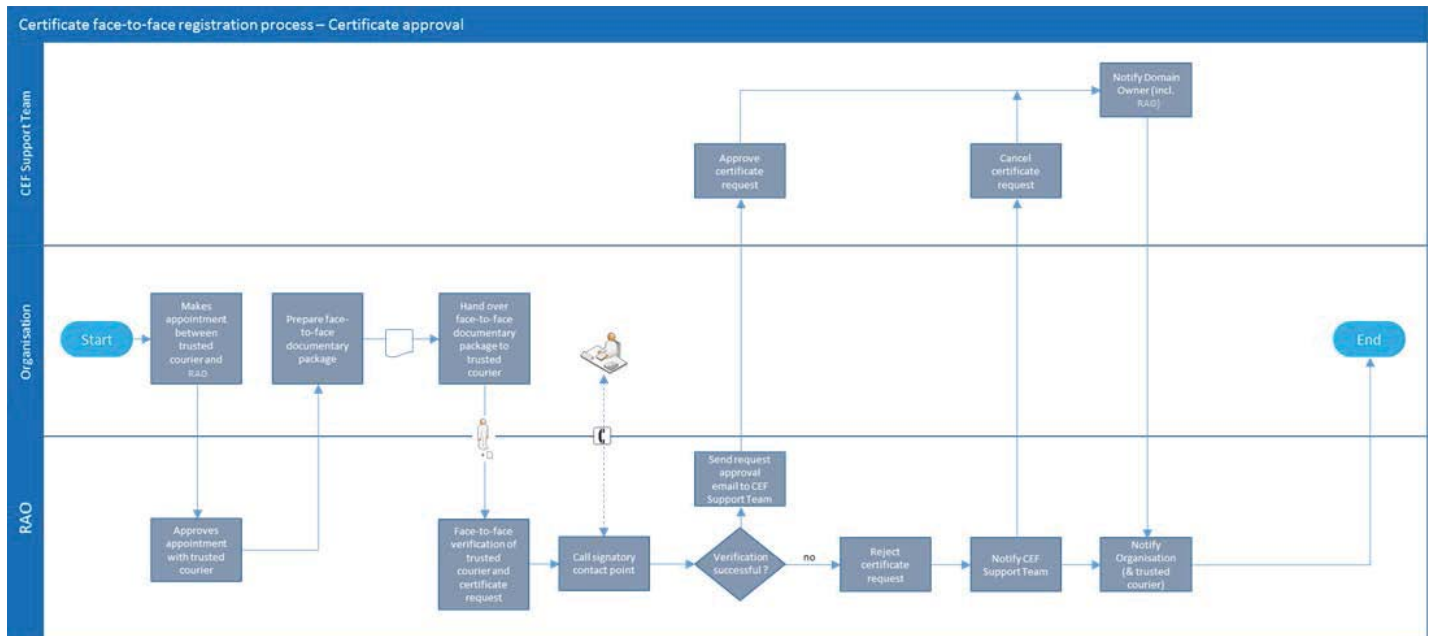
Figure 8 - Certificate approval
