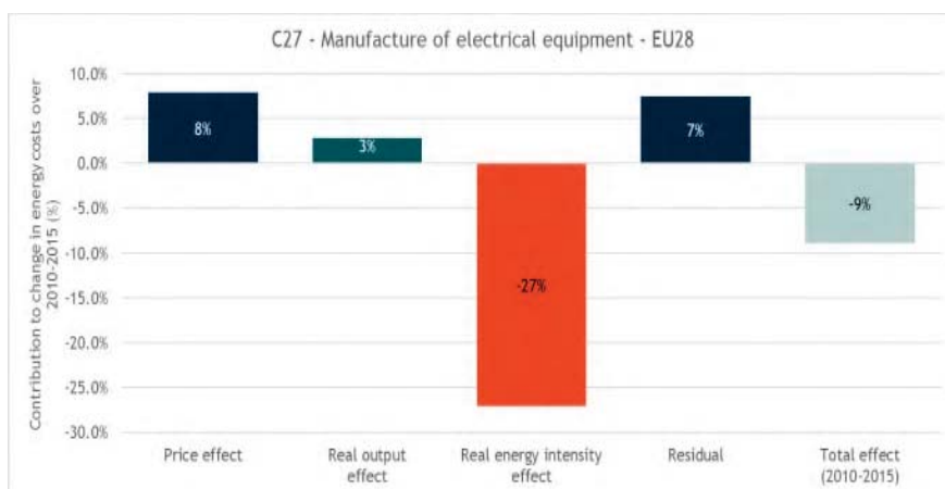
Figure 22: Electrical equipment
