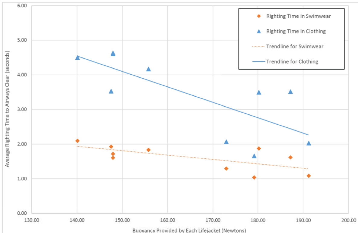
Figure 6: Average righting time versus lifejacket buoyancy
