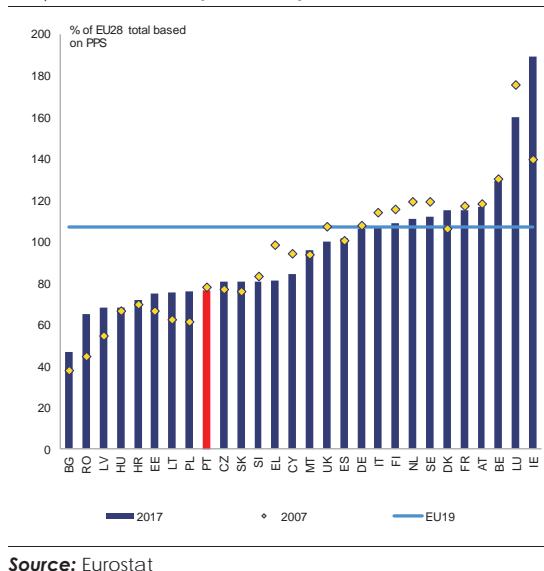
Graph 4.4.1: Labour productivity
