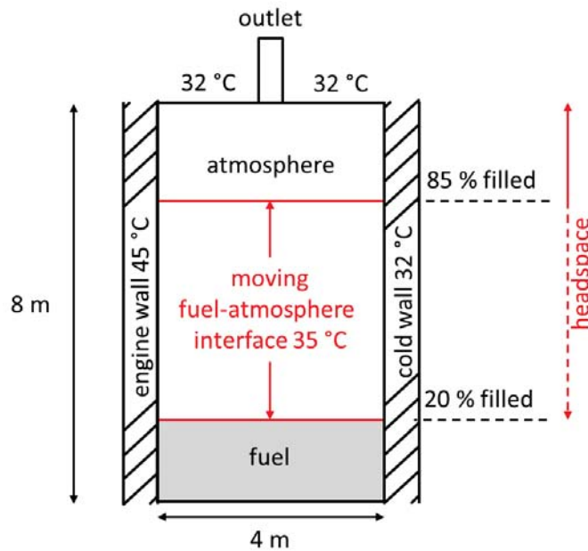
Figure 4 - Geometry of settle tank model
