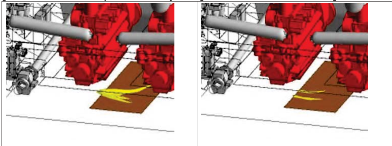
Figure 6 - Position of fuel pools caused by leakage, scenario: 10 m 2 between engines
