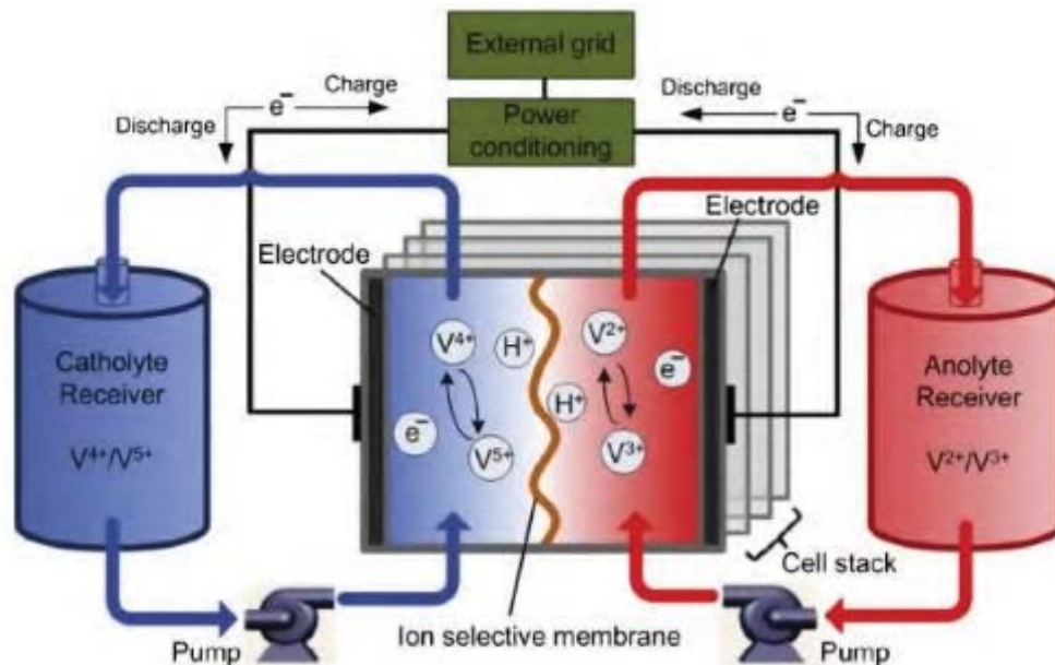
Figure 24: Schematic of vanadium redox flow battery [29]
