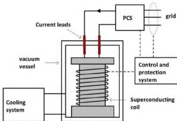
Figure 26: SMES layout [54]
