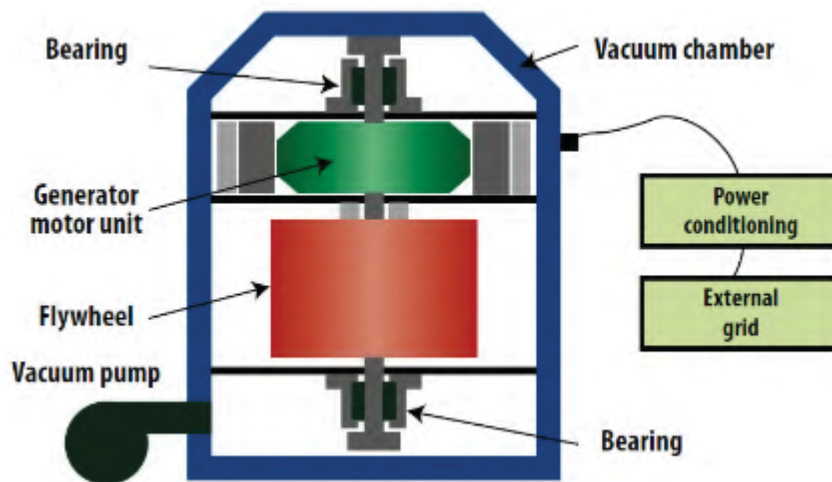
Figure 21: Flywheels layout [29]
