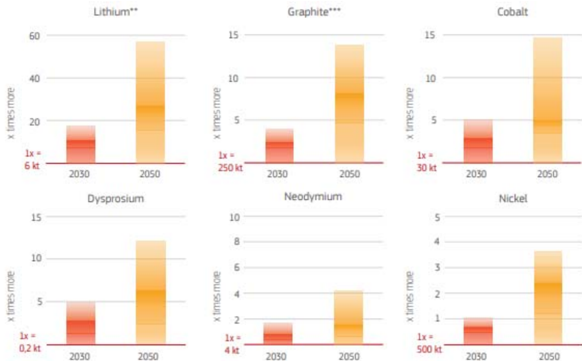
Figure 2: Material consumption for batteries, fuel cells, wind turbines and photovoltaics in 2030 and 2050 as a multiple of current (2020) EU consumption of the material in all applications 211
