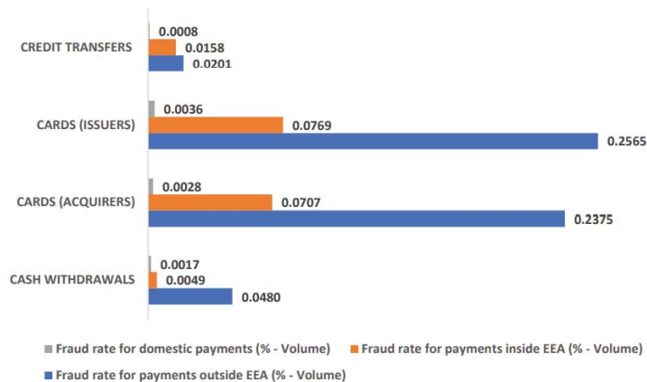
Figure 13: Fraud rate when payments are executed domestically, inside EEA and outside EEA
